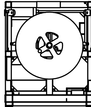
B-B ( 1 : 30 ) Cut thru Section
