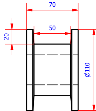
Control Line Oil Roller
